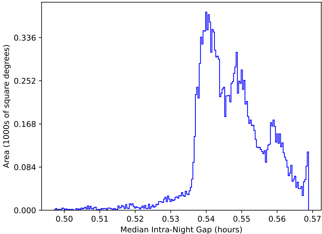
ddf_acor_sf15_ls40_lsr50_v3.4_10yrs WFD: Median Intra-Night Gap
