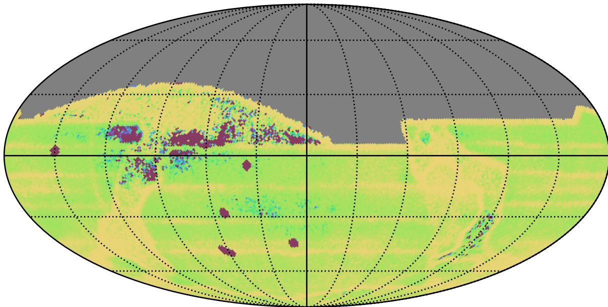
ddf_acor_sf15_lsf40_lsr50_v3.4_10yrs All sky: Median Intra-Night Gap
