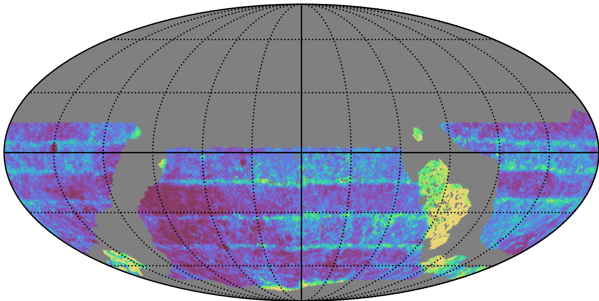
ddf_acor_sf15_lsf40_lsr50_v3.4_10yrs WFD z band: Median Inter-Night Gap
