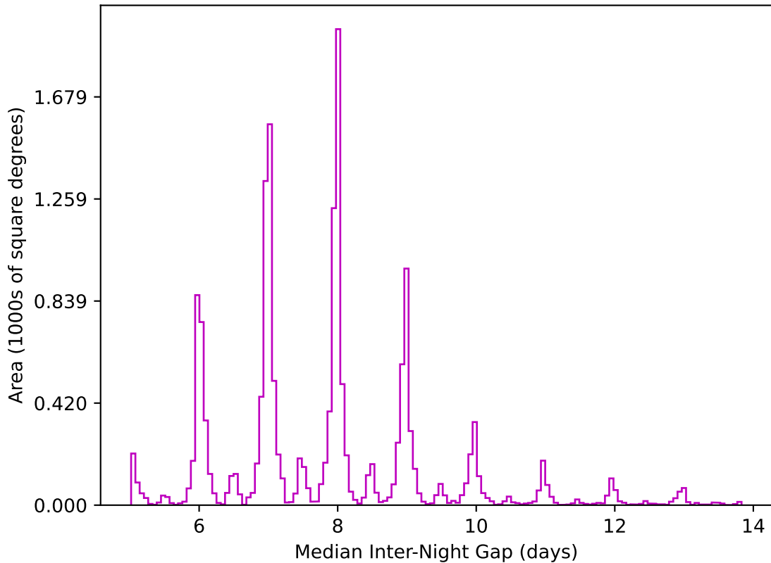
ddf_acor_sf15_lsf40_lsr50_v3.4_10yrs WFD z band: Median Inter-Night Gap
