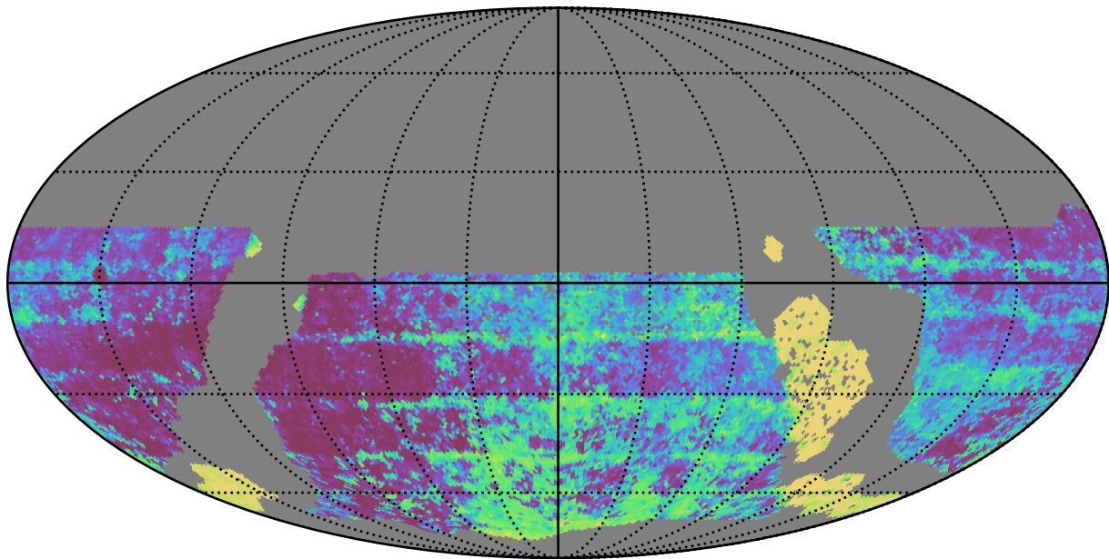
ddf_acor_sf15_lsf40_lsr50_v3.4_10yrs WFD y band: Median Inter-Night Gap
