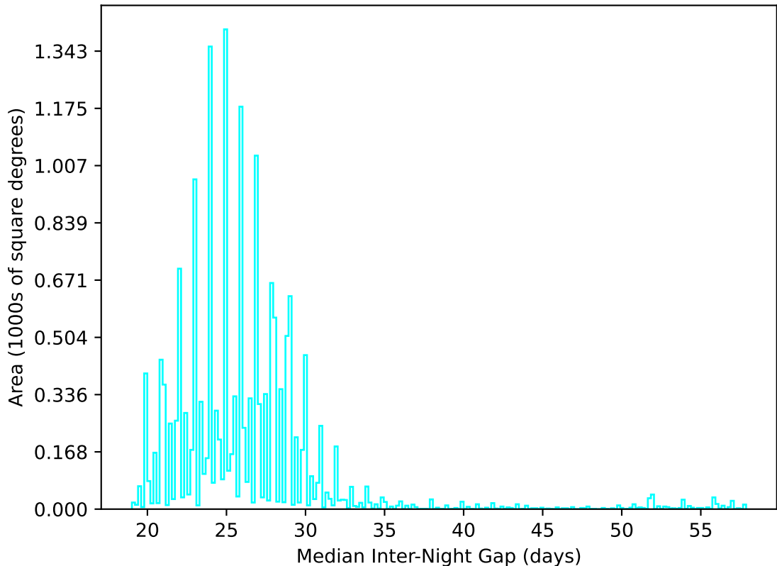
ddf_acor_sf15_lsf40_lsr50_v3.4_10yrs WFD u band: Median Inter-Night Gap
