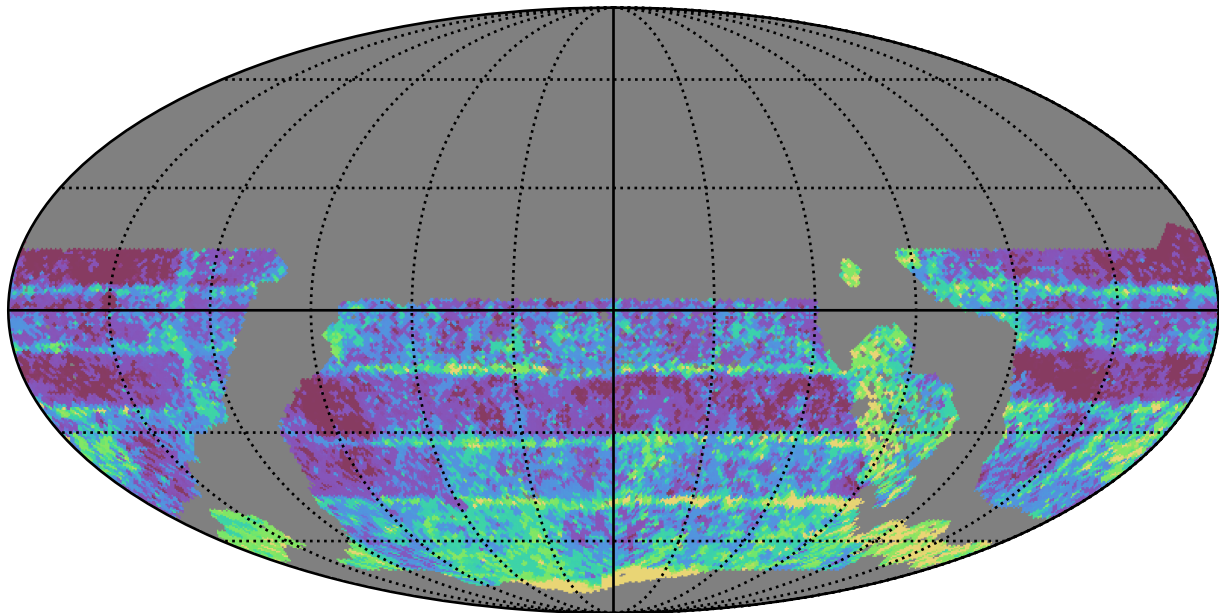
ddf_acor_sf15_lsf40_lsr50_v3.4_10yrs WFD r band: Median Inter-Night Gap
