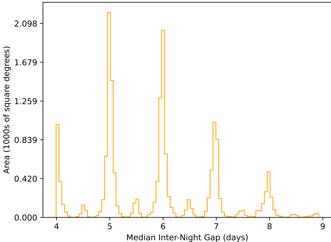
ddf_acor_sf15_ls40_lsr50_v3.4_10yrs WFD r band: Median Inter-Night Gap
