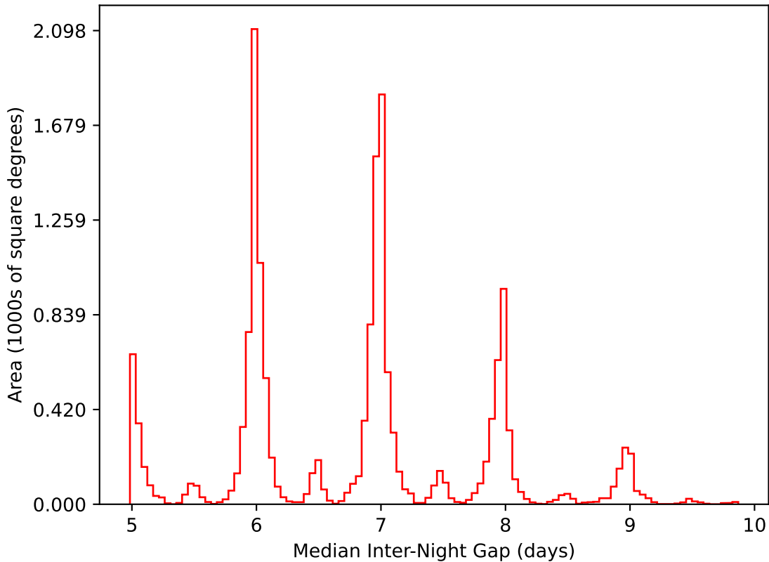
ddf_acor_sf15_lsf40_lsr50_v3.4_10yrs WFD i band: Median Inter-Night Gap
