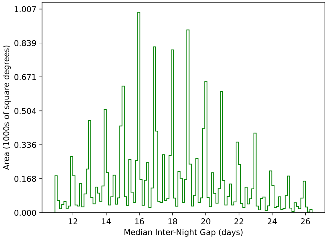
ddf_acor_sf15_lsf40_lsr50_v3.4_10yrs WFD g band: Median Inter-Night Gap
