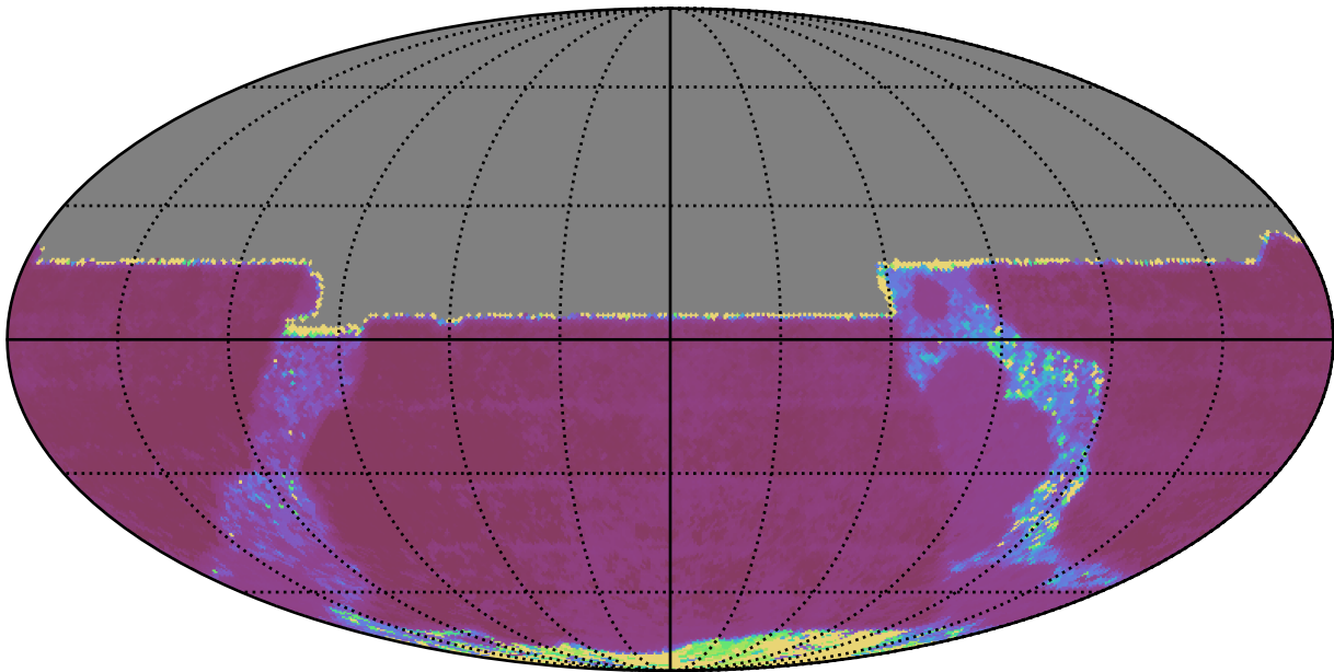
ddf_acor_sf15_lsf40_lsr50_v3.4_10yrs All sky y band: Median Inter-Night Gap
