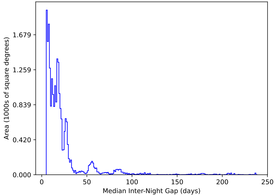
ddf_acor_sf15_lsf40_lsr50_v3.4_10yrs All sky y band: Median Inter-Night Gap
