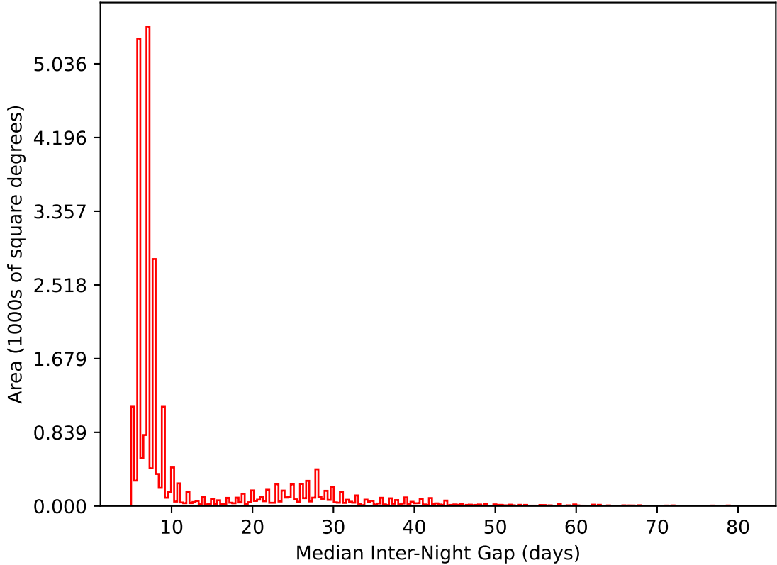
ddf_acor_sf15_lsf40_lsr50_v3.4_10yrs All sky i band: Median Inter-Night Gap
