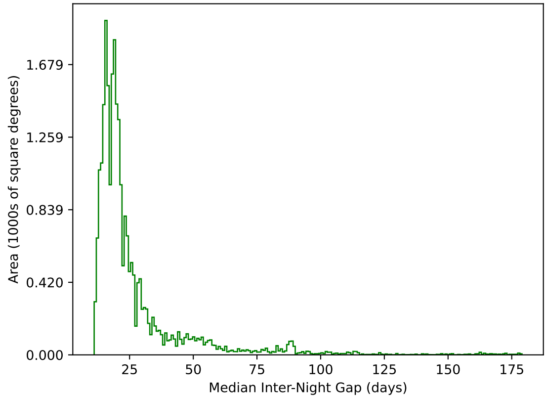
ddf_acor_sf15_lsf40_lsr50_v3.4_10yrs All sky g band: Median Inter-Night Gap
