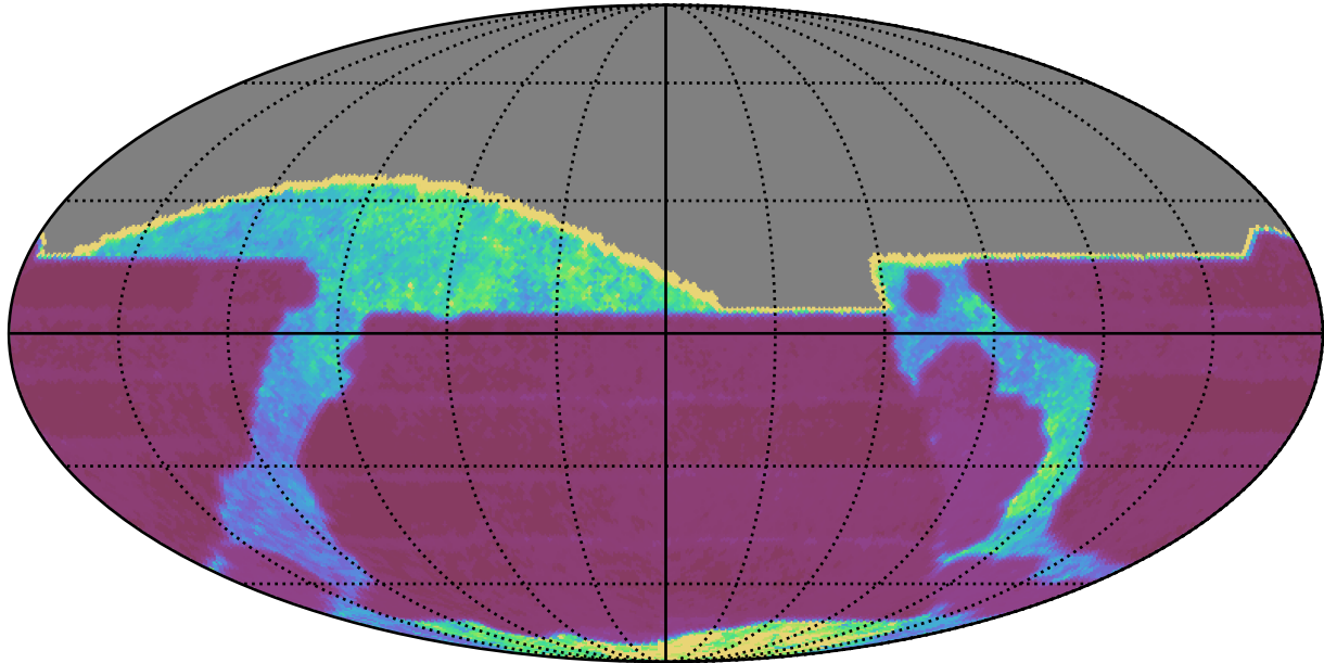
ddf_acor_sf15_lsf40_lsr50_v3.4_10yrs All sky all bands: Median Inter-Night Gap
