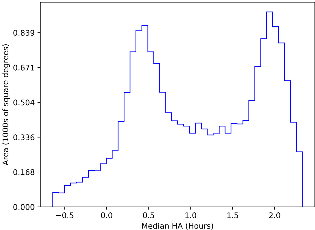
ddf_acor_sf15_lsf40_lsr50_v3.4_10yrs WFD z band: Median HA
