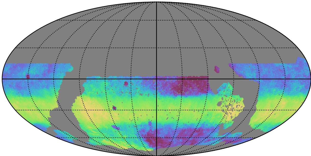
ddf_acor_sf15_lsf40_lsr50_v3.4_10yrs WFD y band: Median HA
