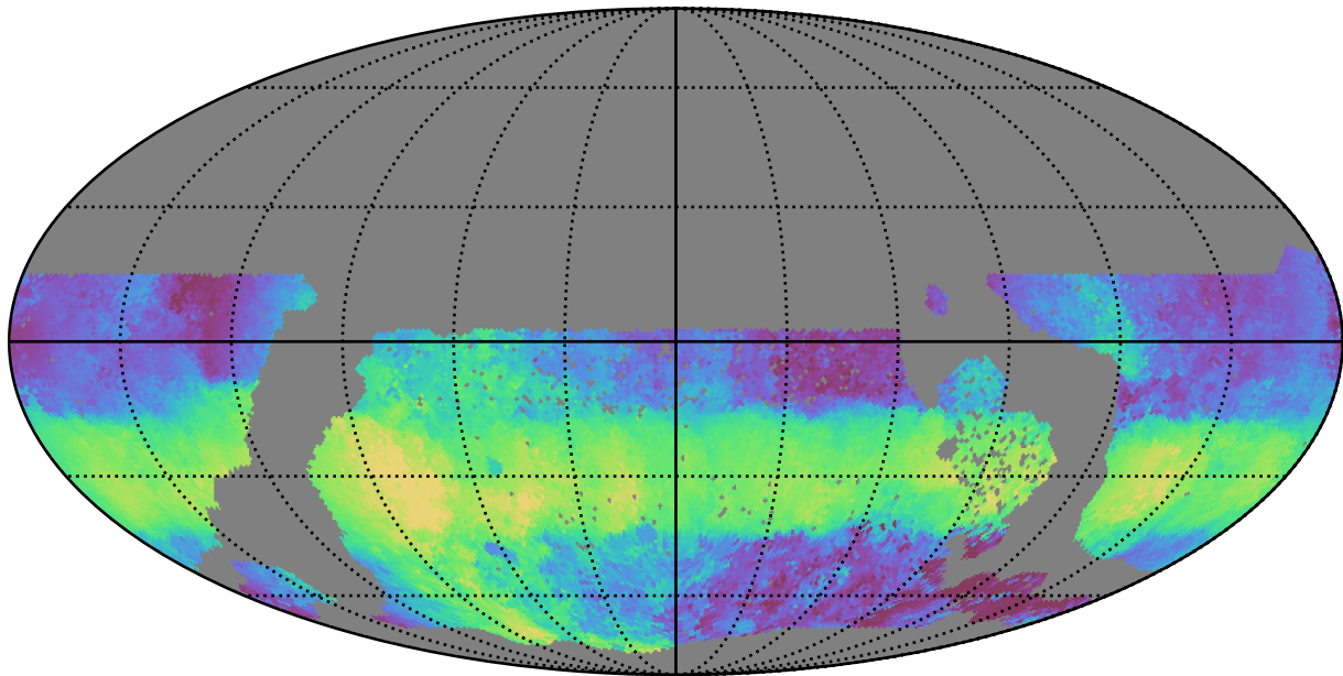
ddf_acor_sf15_lsf40_lsr50_v3.4_10yrs WFD u band: Median HA
