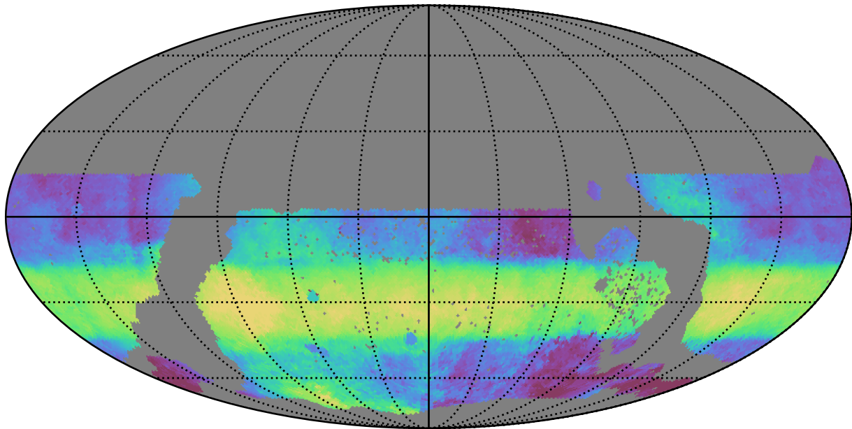
ddf_acor_sf15_lsf40_lsr50_v3.4_10yrs WFD r band: Median HA
