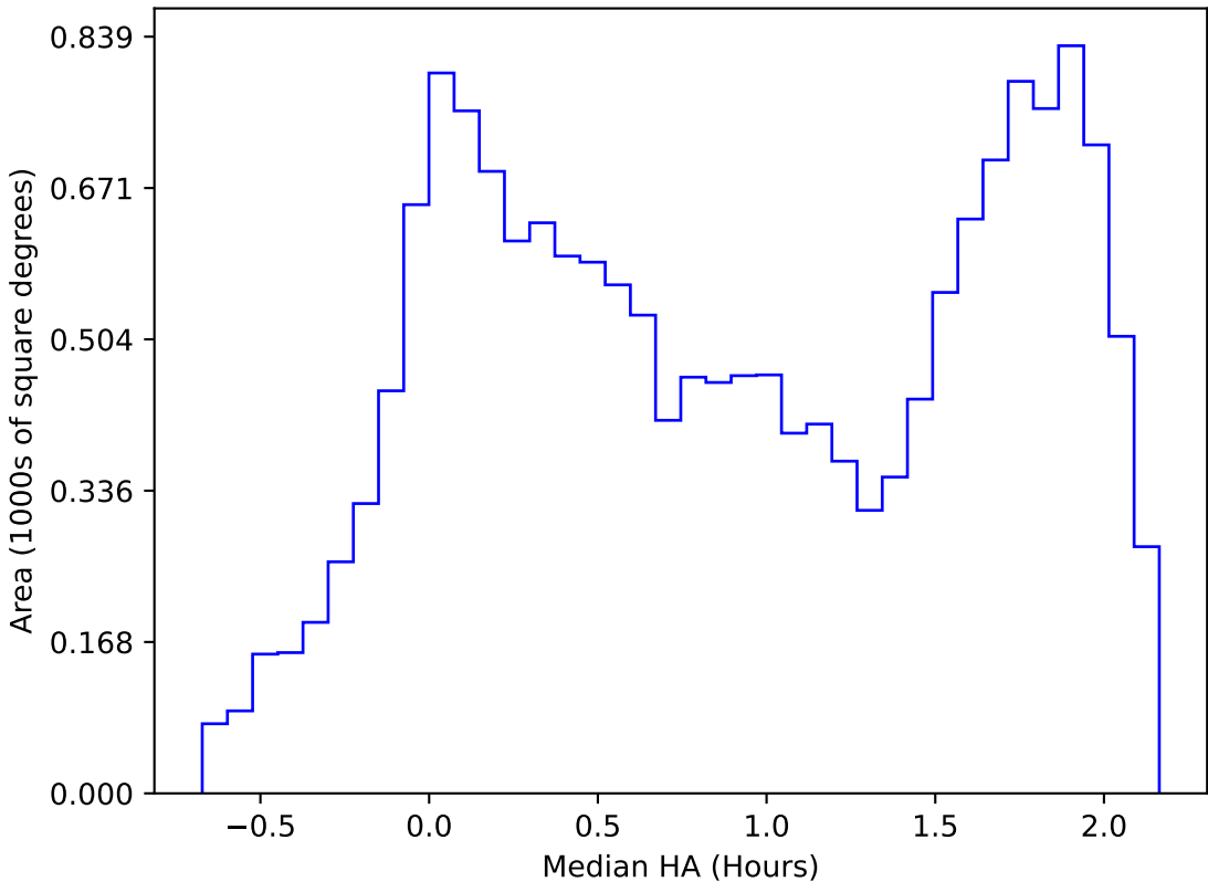
ddf_acor_sf15_lsf40_lsr50_v3.4_10yrs WFD r band: Median HA
