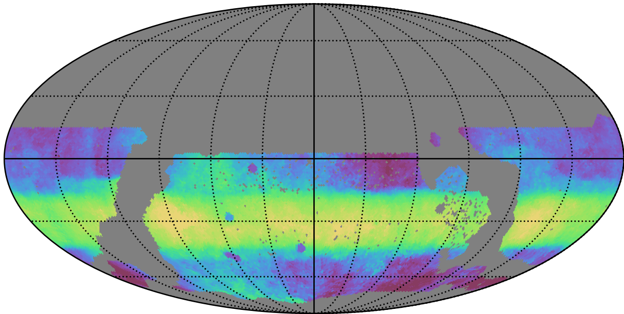
ddf_acor_sf15_lsf40_lsr50_v3.4_10yrs WFD i band: Median HA
