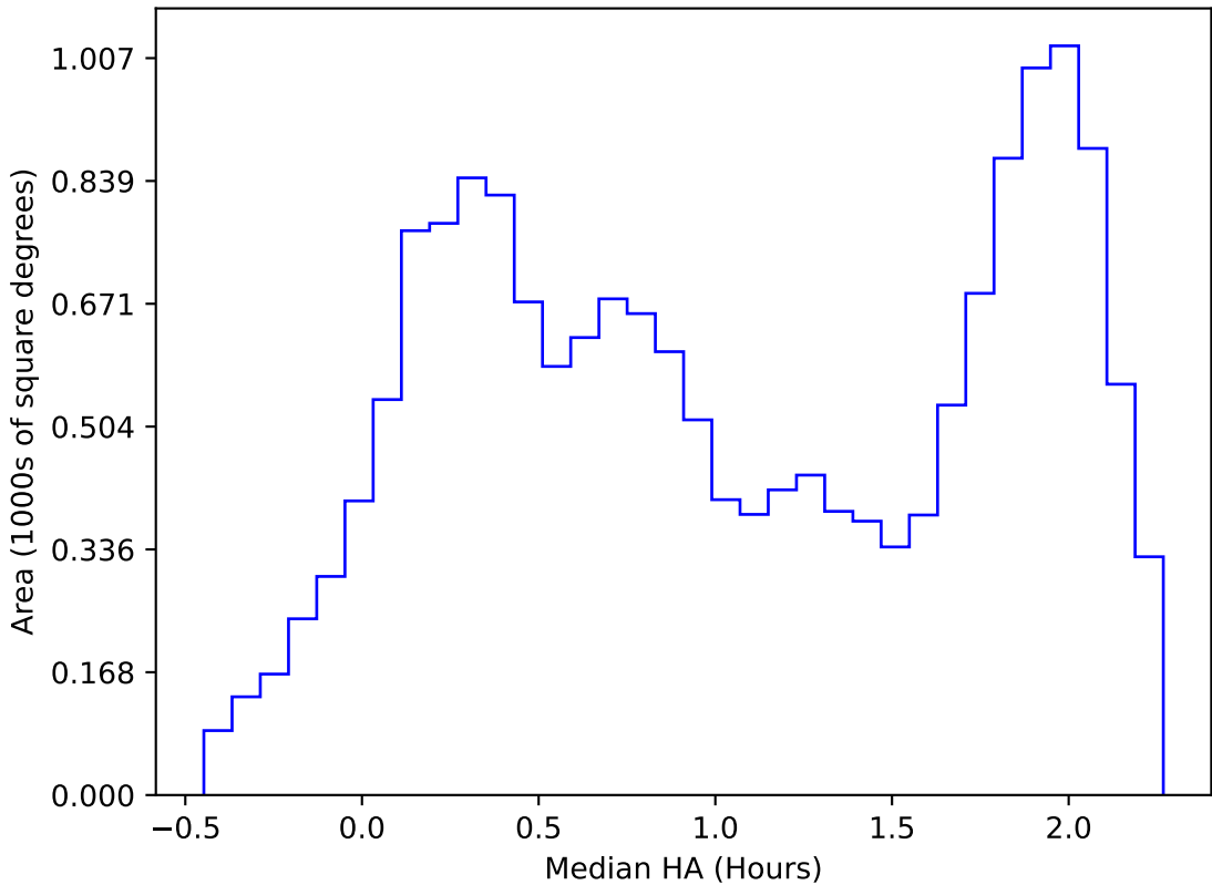
ddf_acor_sf15_lsf40_lsr50_v3.4_10yrs WFD i band: Median HA
