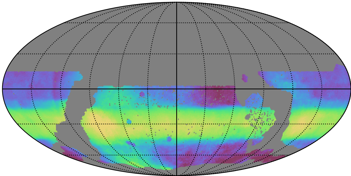
ddf_acor_sf15_lsf40_lsr50_v3.4_10yrs WFD all bands: Median HA
