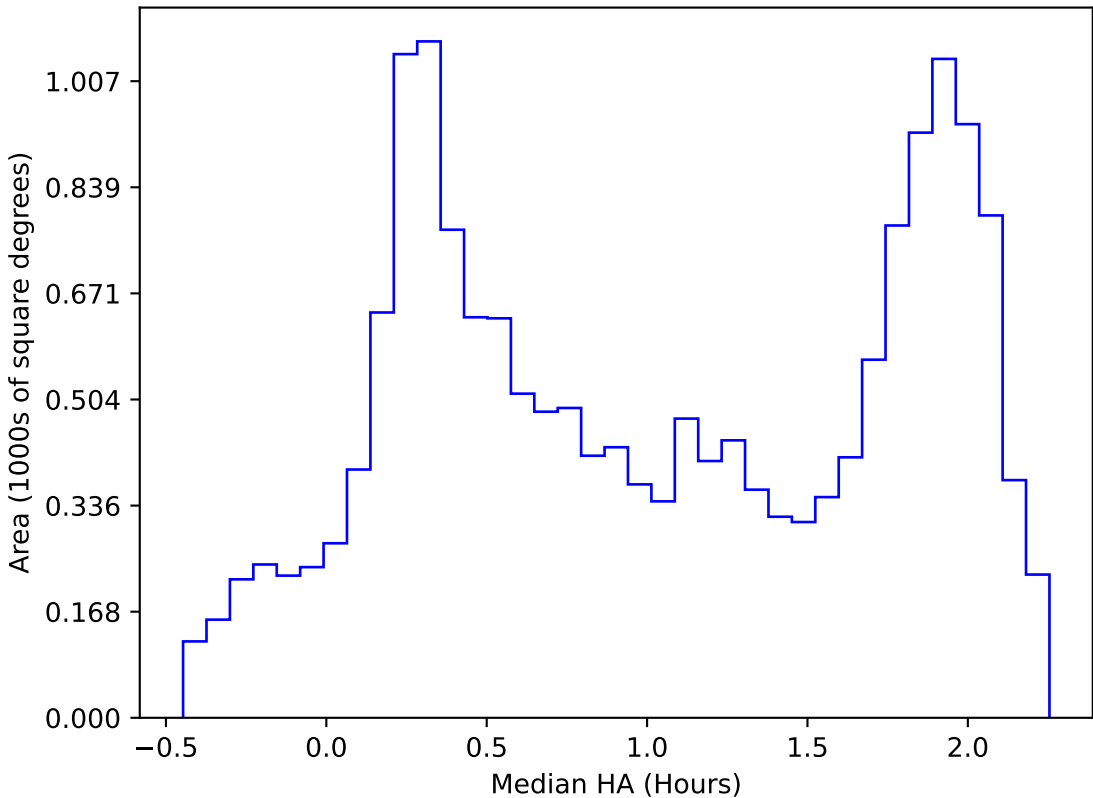
ddf_acor_sf15_lsf40_lsr50_v3.4_10yrs WFD all bands: Median HA
