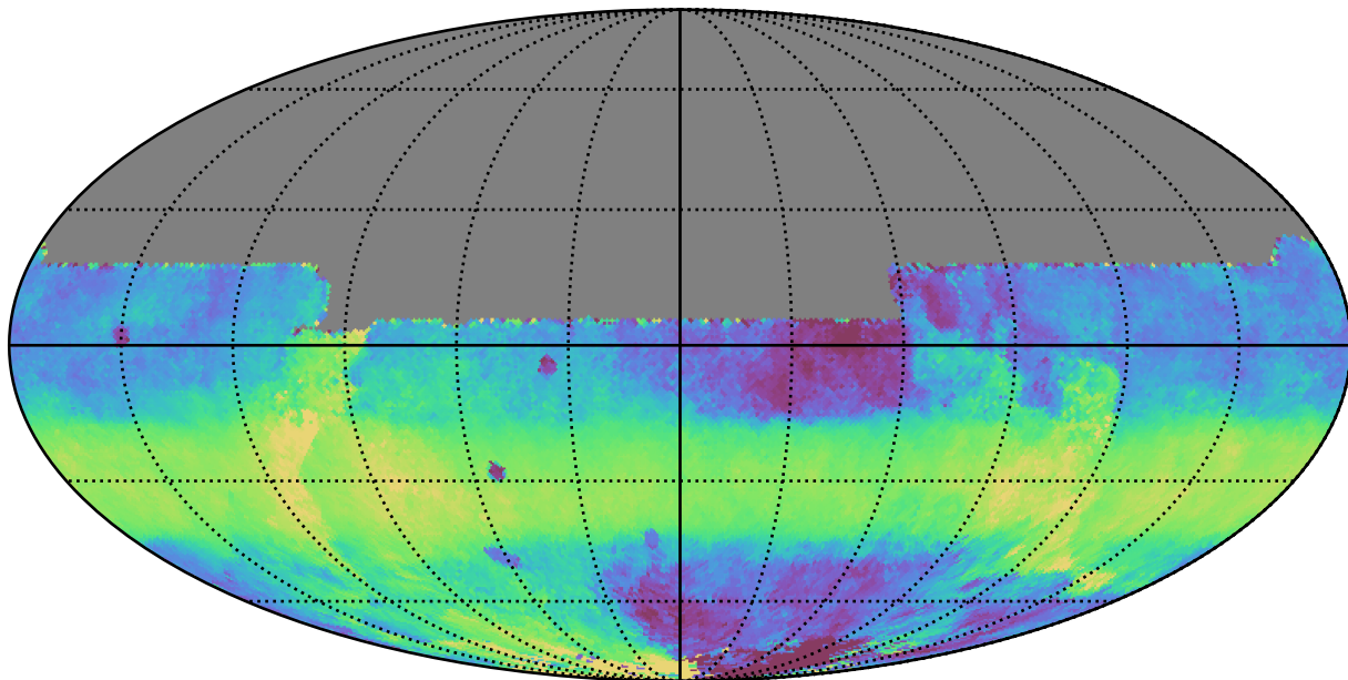
ddf_acor_sf15_lsf40_lsr50_v3.4_10yrs All sky y band: Median HA
