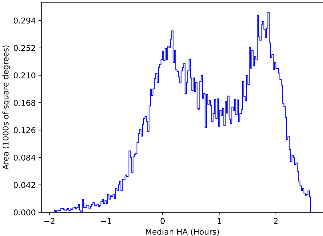
ddf_acor_sf15_lsf40_lsr50_v3.4_10yrs All sky u band: Median HA
