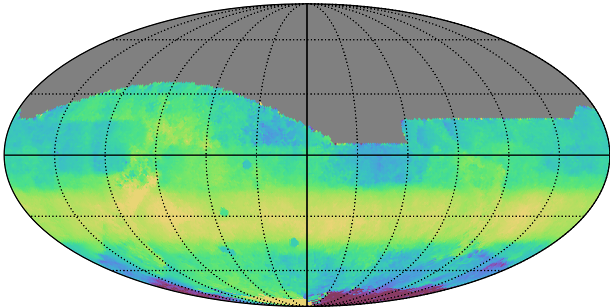
ddf_acor_sf15_lsf40_lsr50_v3.4_10yrs All sky i band: Median HA
