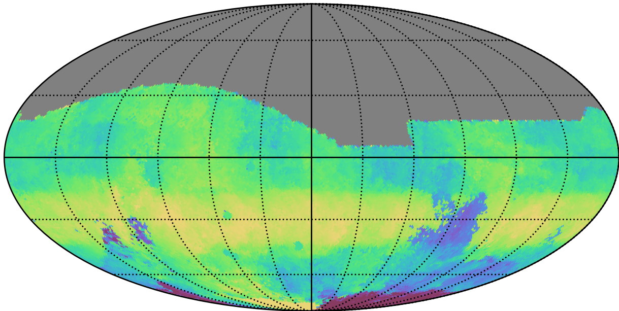
ddf_acor_sf15_lsf40_lsr50_v3.4_10yrs All sky g band: Median HA
