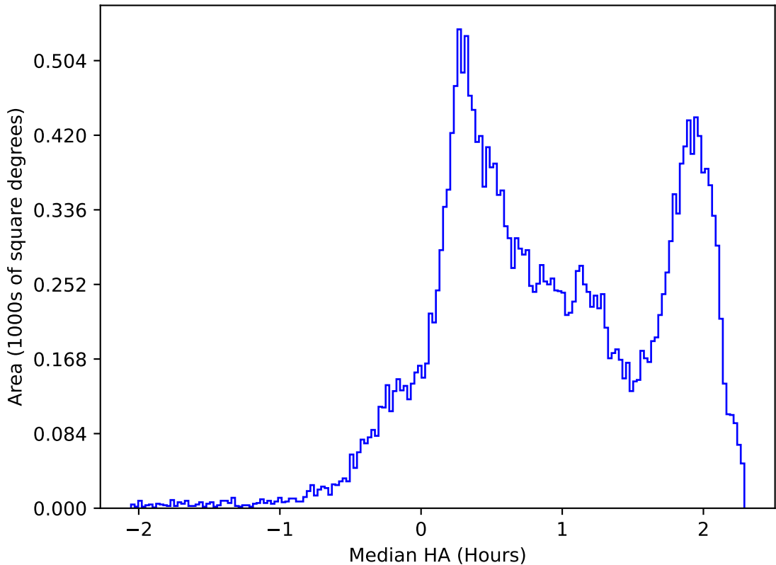
ddf_acor_sf15_lsf40_lsr50_v3.4_10yrs All sky all bands: Median HA
