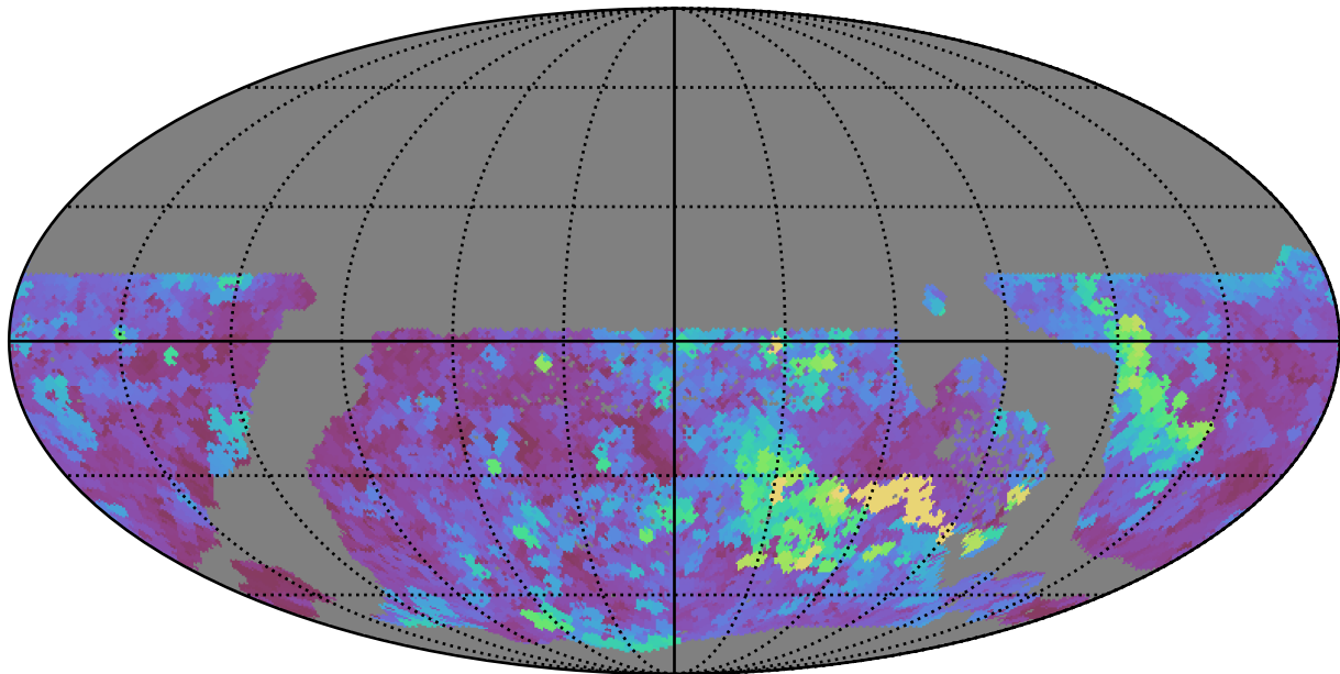
ddf_acor_sf15_lsf40_lsr50_v3.4_10yrs WFD u band: Max seeingEff
