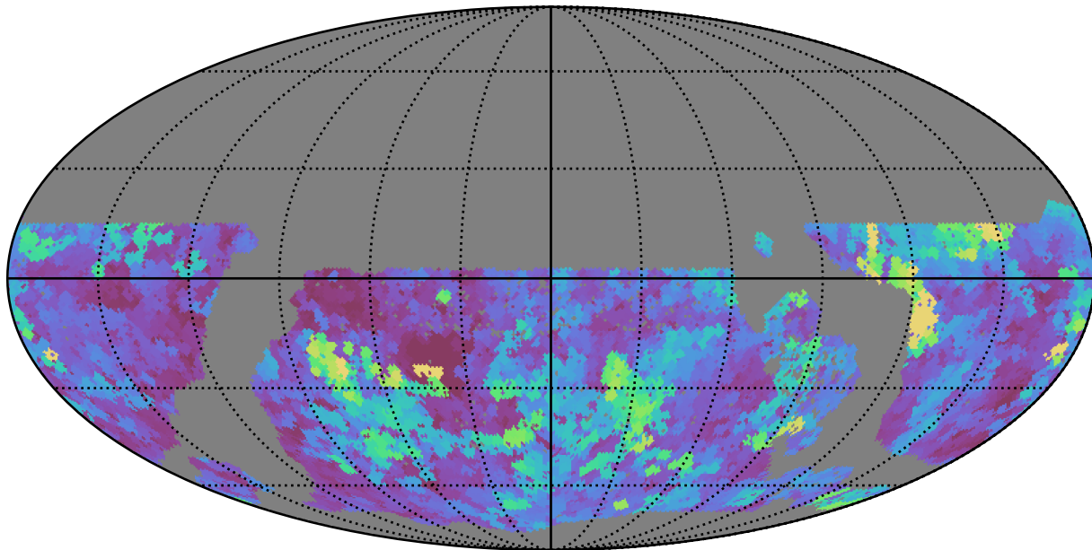
ddf_acor_sf15_lsf40_lsr50_v3.4_10yrs WFD g band: Max seeingEff
