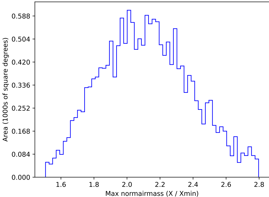
ddf_acor_sf15_lsf40_lsr50_v3.4_10yrs WFD y band: Max normairmass
