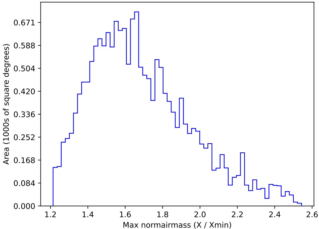
ddf_acor_sf15_lsf40_lsr50_v3.4_10yrs WFD u band: Max normairmass
