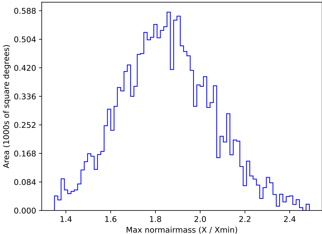
ddf_acor_sf15_lsf40_lsr50_v3.4_10yrs WFD g band: Max normairmass
