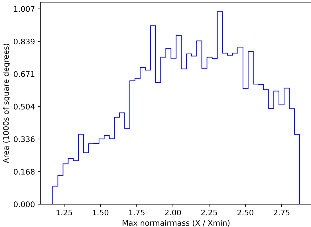
ddf_acor_sf15_lsf40_lsr50_v3.4_10yrs All sky i band: Max normairmass
