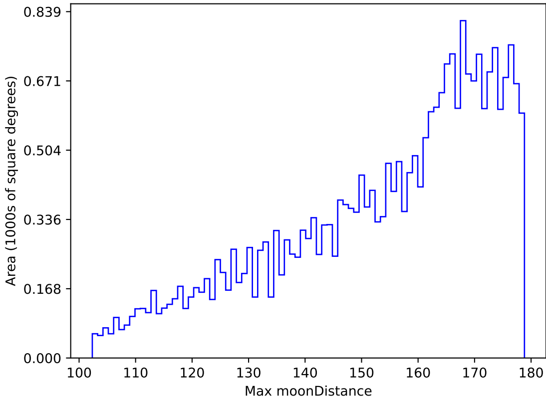
ddf_acor_sf15_lsf40_lsr50_v3.4_10yrs All sky z band: Max moonDistance
