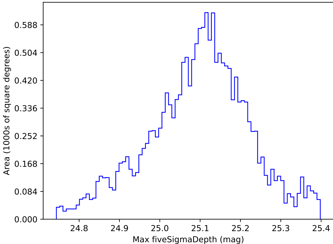
ddf_acor_sf15_lsf40_lsr50_v3.4_10yrs WFD all bands: Max fiveSigmaDepth
