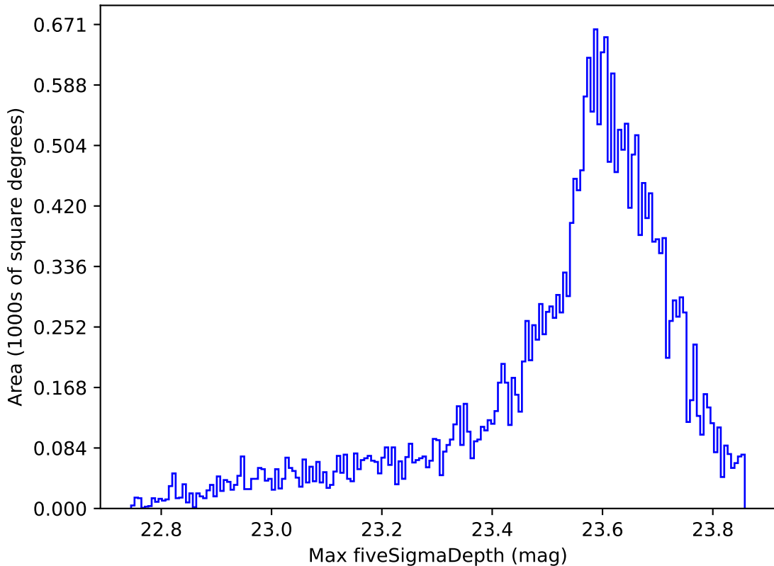
ddf_acor_sf15_lsf40_lsr50_v3.4_10yrs All sky z band: Max fiveSigmaDepth
