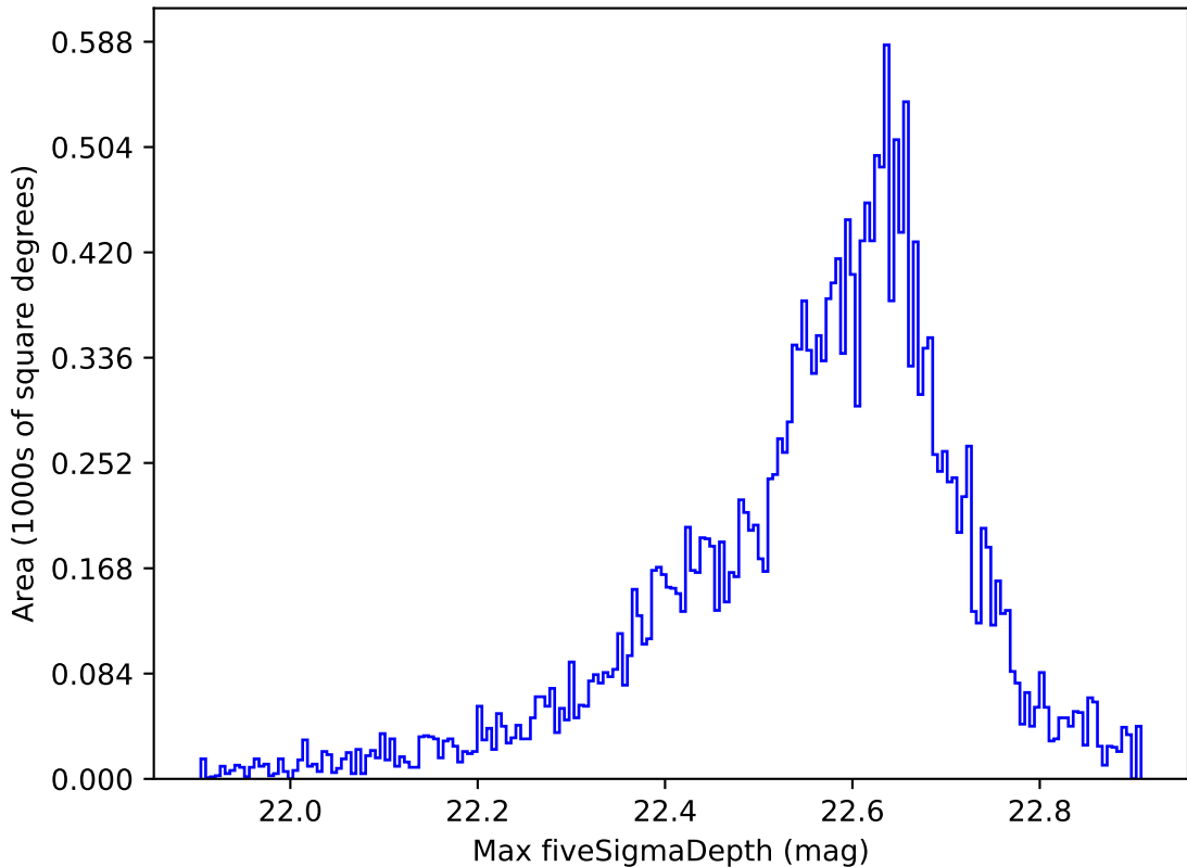
ddf_acor_sf15_lsf40_lsr50_v3.4_10yrs All sky y band: Max fiveSigmaDepth
