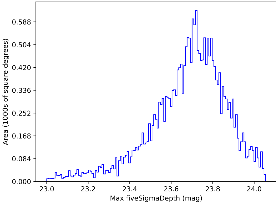
ddf_acor_sf15_ls40_lsr50_v3.4_10yrs All sky u band: Max fiveSigmaDepth
