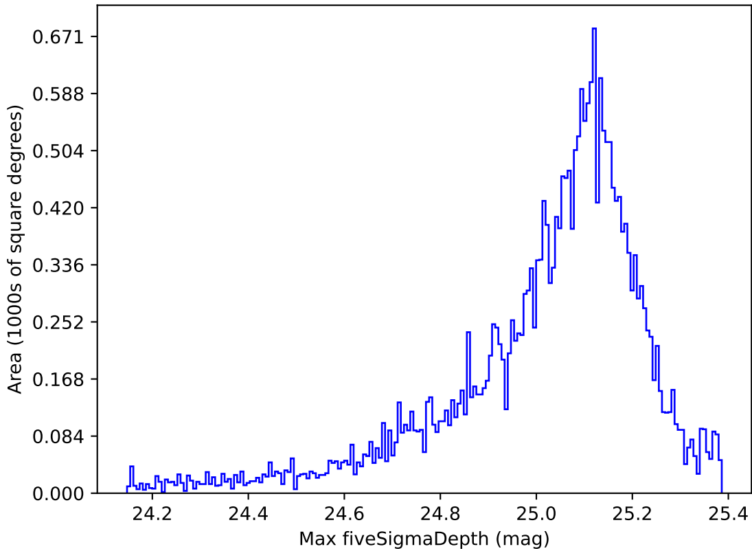
ddf_acor_sf15_lsf40_lsr50_v3.4_10yrs All sky g band: Max fiveSigmaDepth
