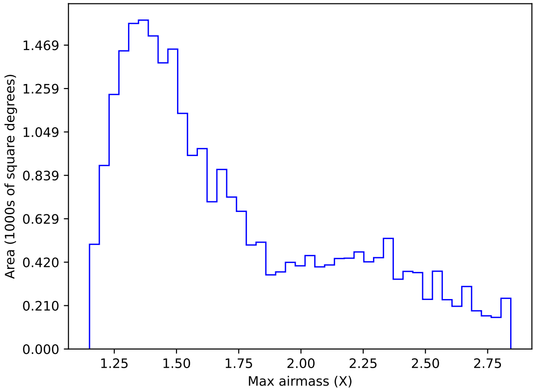
ddf_acor_sf15_lsf40_lsr50_v3.4_10yrs Yr 1 z band: Max airmass
