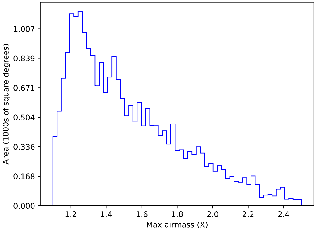
ddf_acor_sf15_lsf40_lsr50_v3.4_10yrs Yr 1 u band: Max airmass
