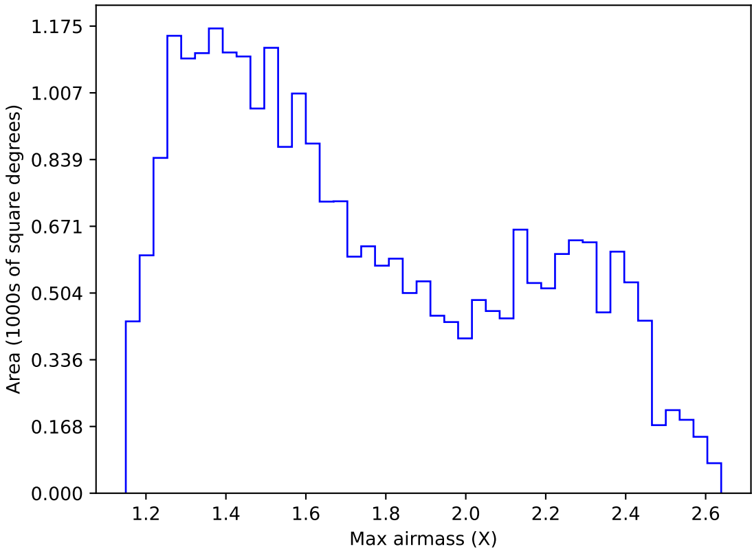
ddf_acor_sf15_lsf40_lsr50_v3.4_10yrs Yr 1 r band: Max airmass
