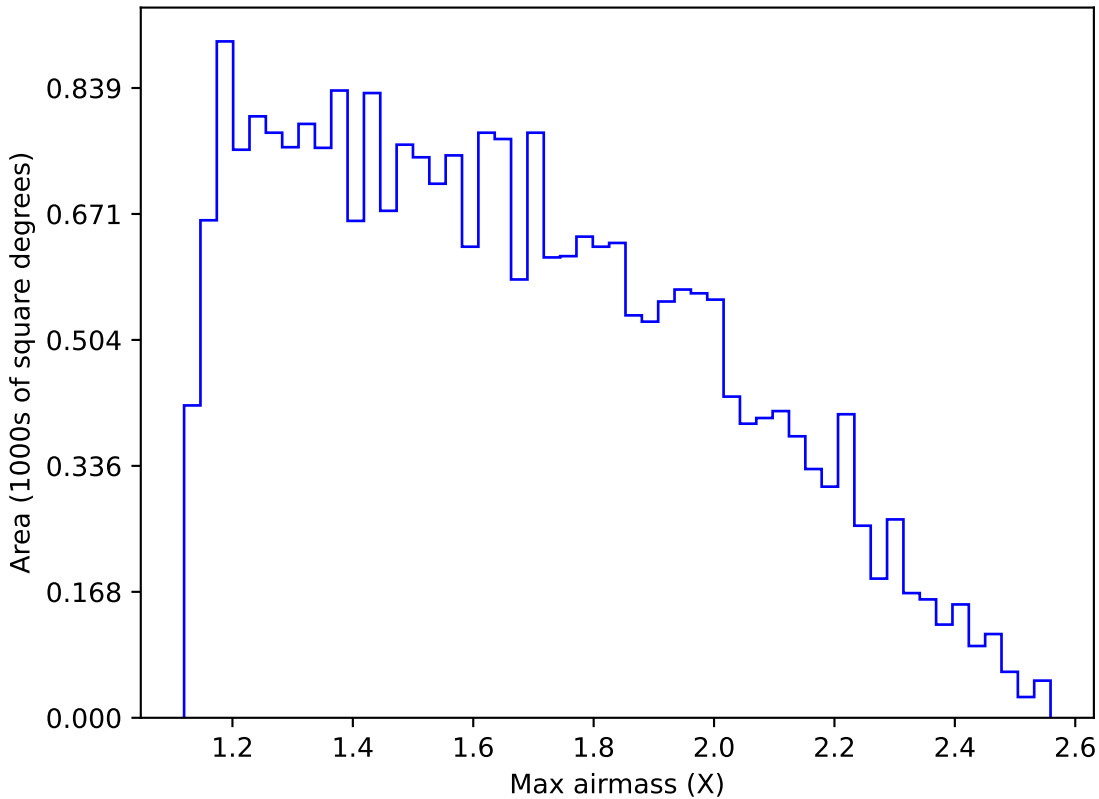
ddf_acor_sf15_lsf40_lsr50_v3.4_10yrs Yr 1 g band: Max airmass
