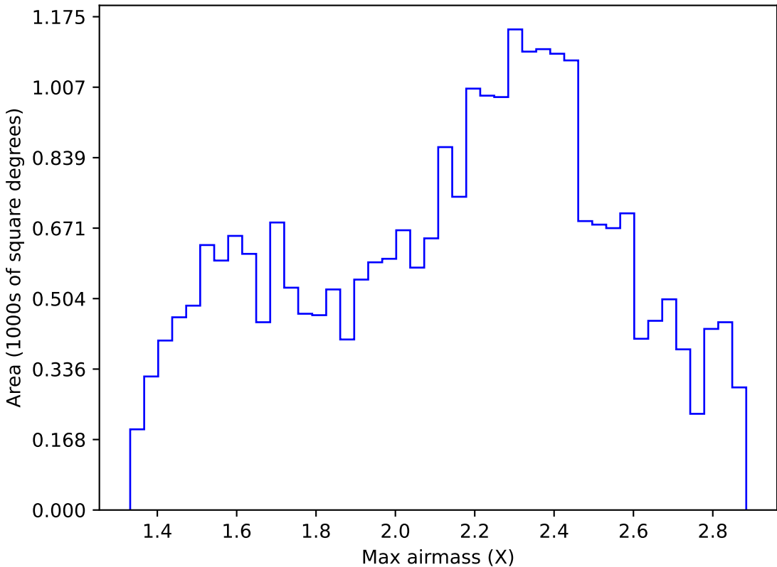
ddf_acor_sf15_lsf40_lsr50_v3.4_10yrs Yr 1 all bands: Max airmass
