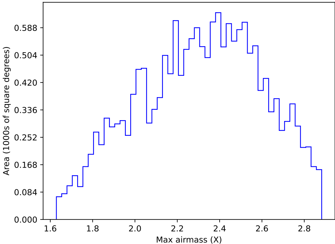
ddf_acor_sf15_lsf40_lsr50_v3.4_10yrs WFD y band: Max airmass
