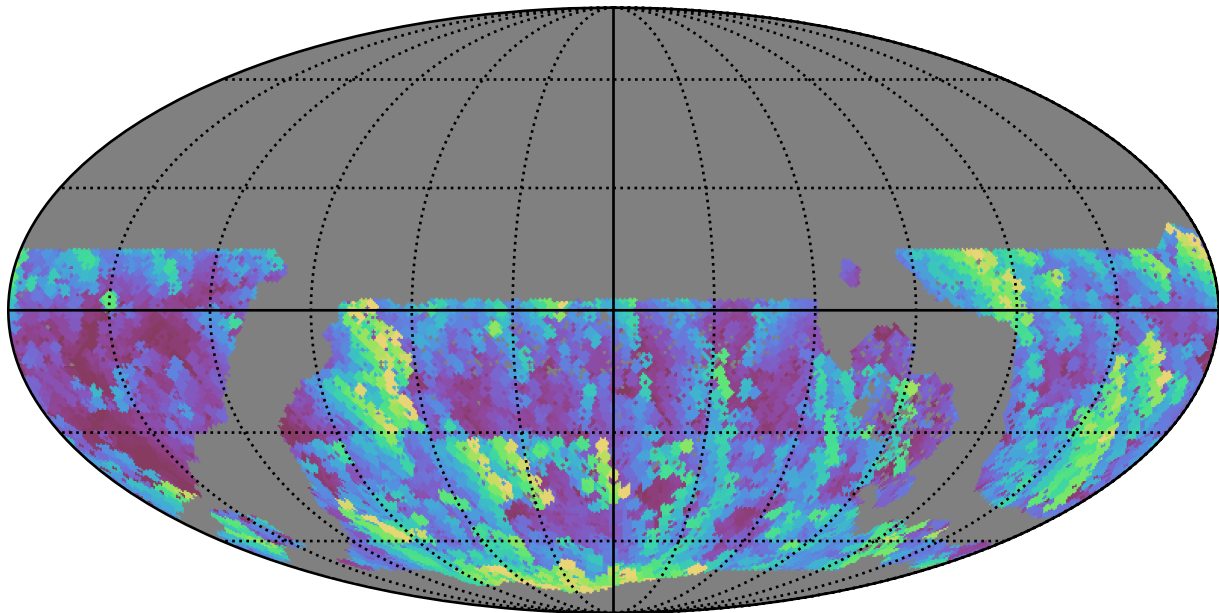
ddf_acor_sf15_lsf40_lsr50_v3.4_10yrs WFD u band: Max airmass
