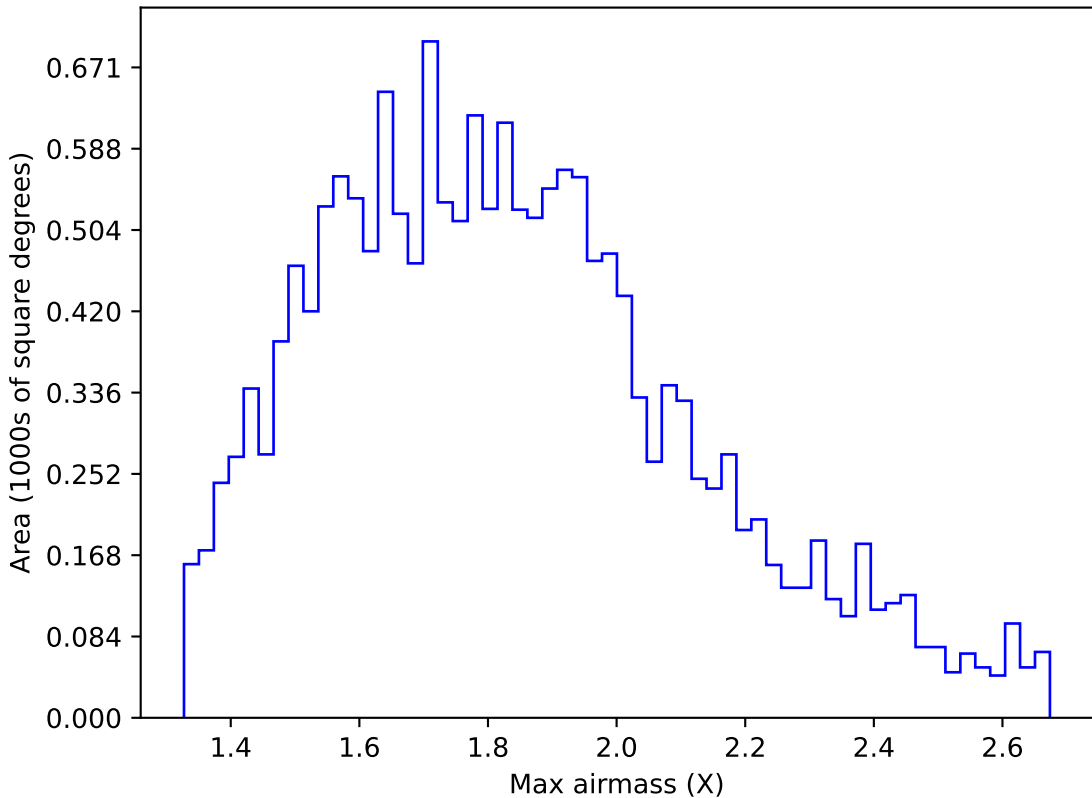
ddf_acor_sf15_lsf40_lsr50_v3.4_10yrs WFD u band: Max airmass
