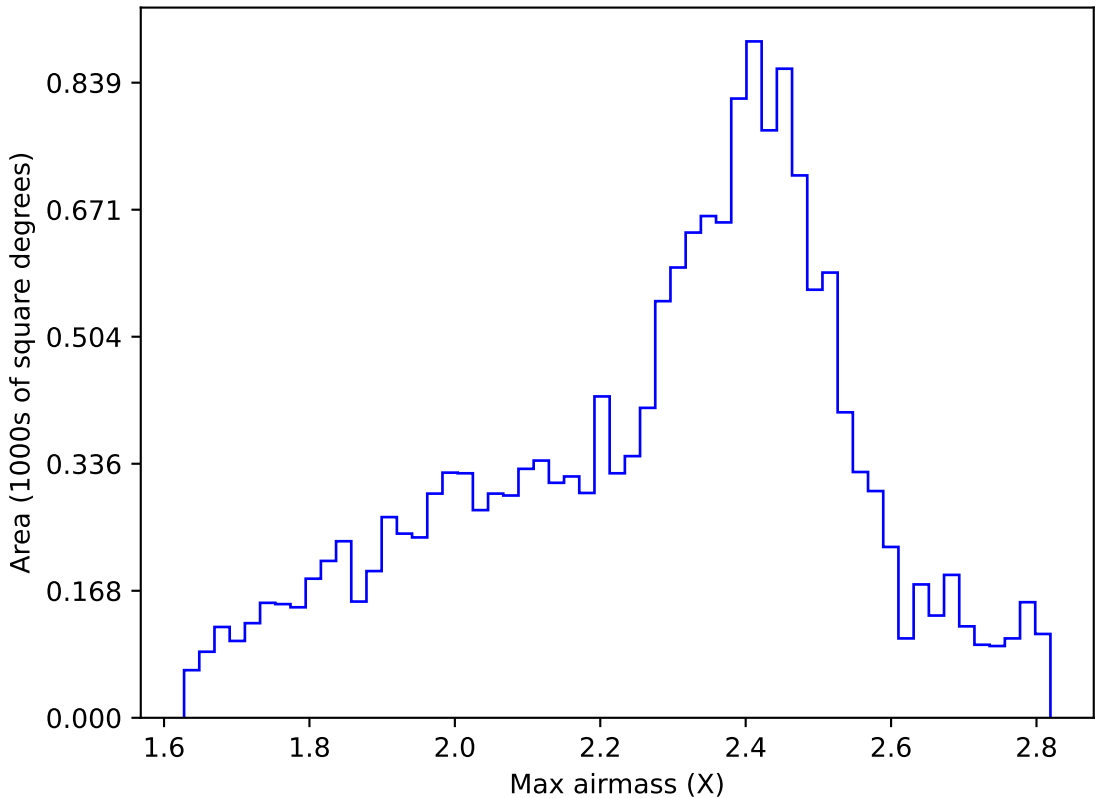
ddf_acor_sf15_lsf40_lsr50_v3.4_10yrs WFD r band: Max airmass
